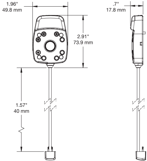
Series 3000 Handheld Sensor Apple Lightning (DWH203-W):
