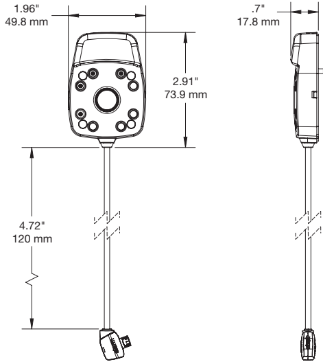
Series 3000 Tablet Sensor Micro USB (DWT200-W):
